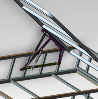
1128-M0148 AMORTİSÖRLÜ BAZA MEKANİZMASI MECHANISM WITH GAS SPRING
